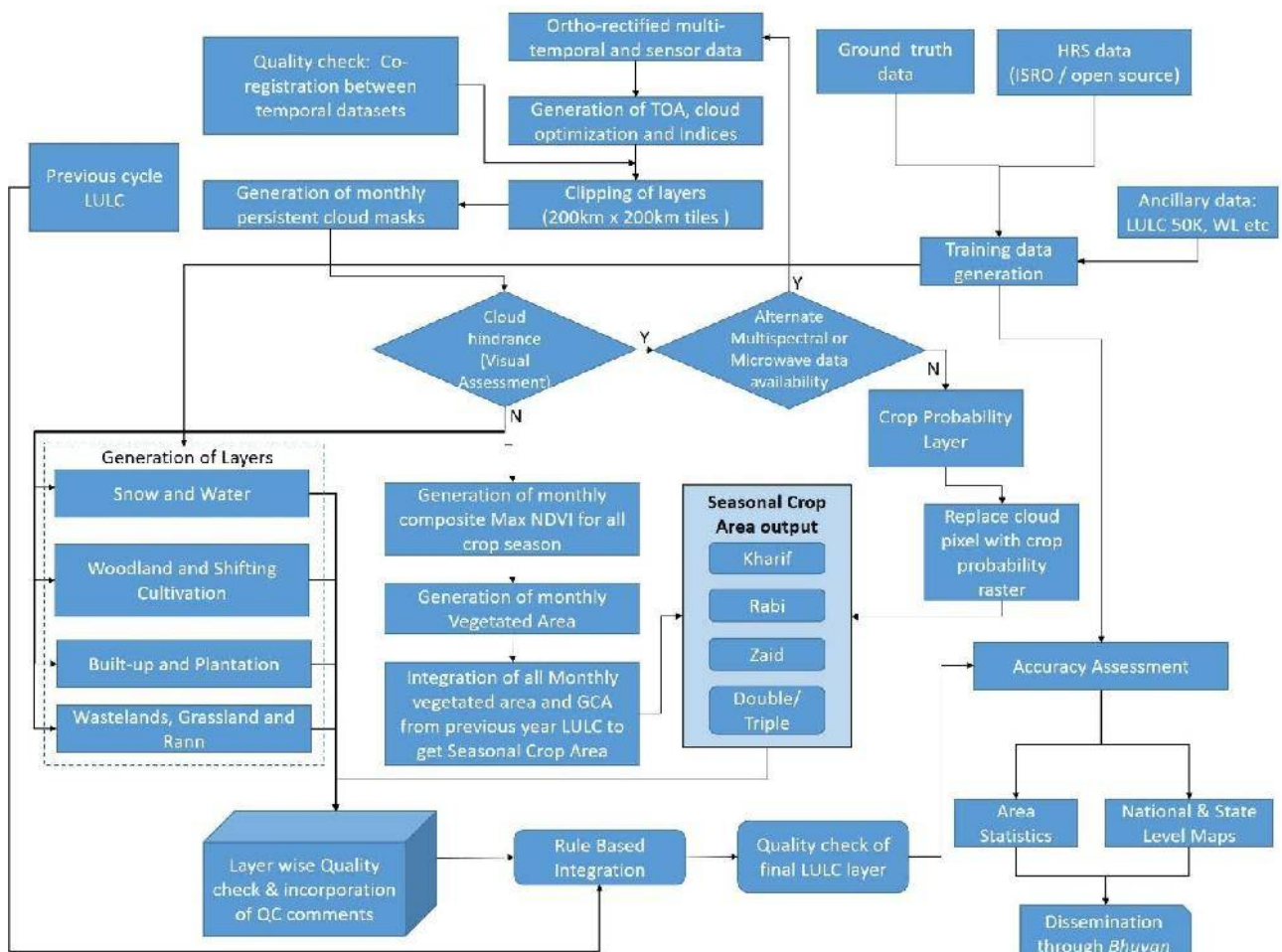
Figure 2- Methodology Flowchart
