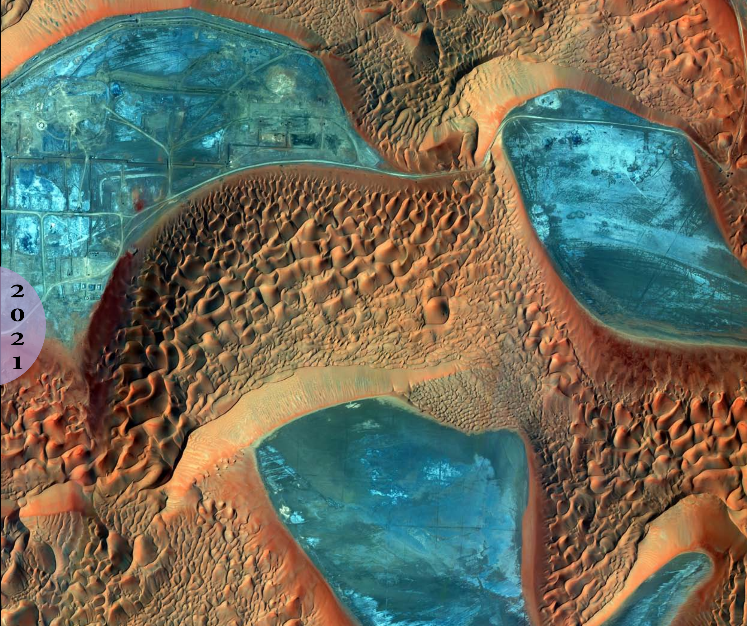
Compound and complex mega-barchan dunes in northeastern margin of Rub Al Khali sand sea, Saudi Arabia. Dunes are surrounded by interdunal depressions with sabkha deposits with patches of gypcrete.
