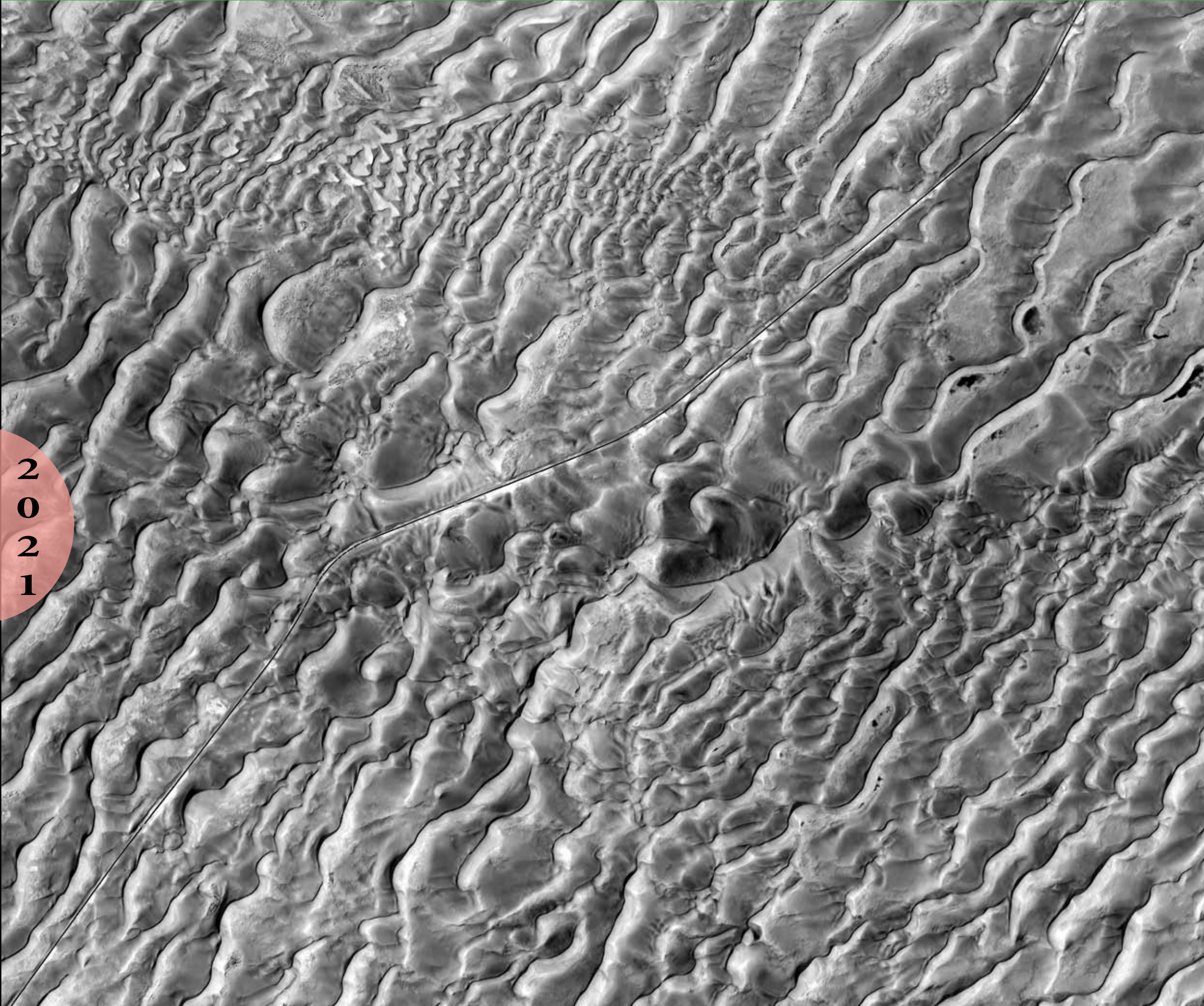
Compound transverse mega dunes and barchanoid dunes in eastern Gobi Desert, south of Mangolia. At places, star dunes also have developed under a variable wind regime.
