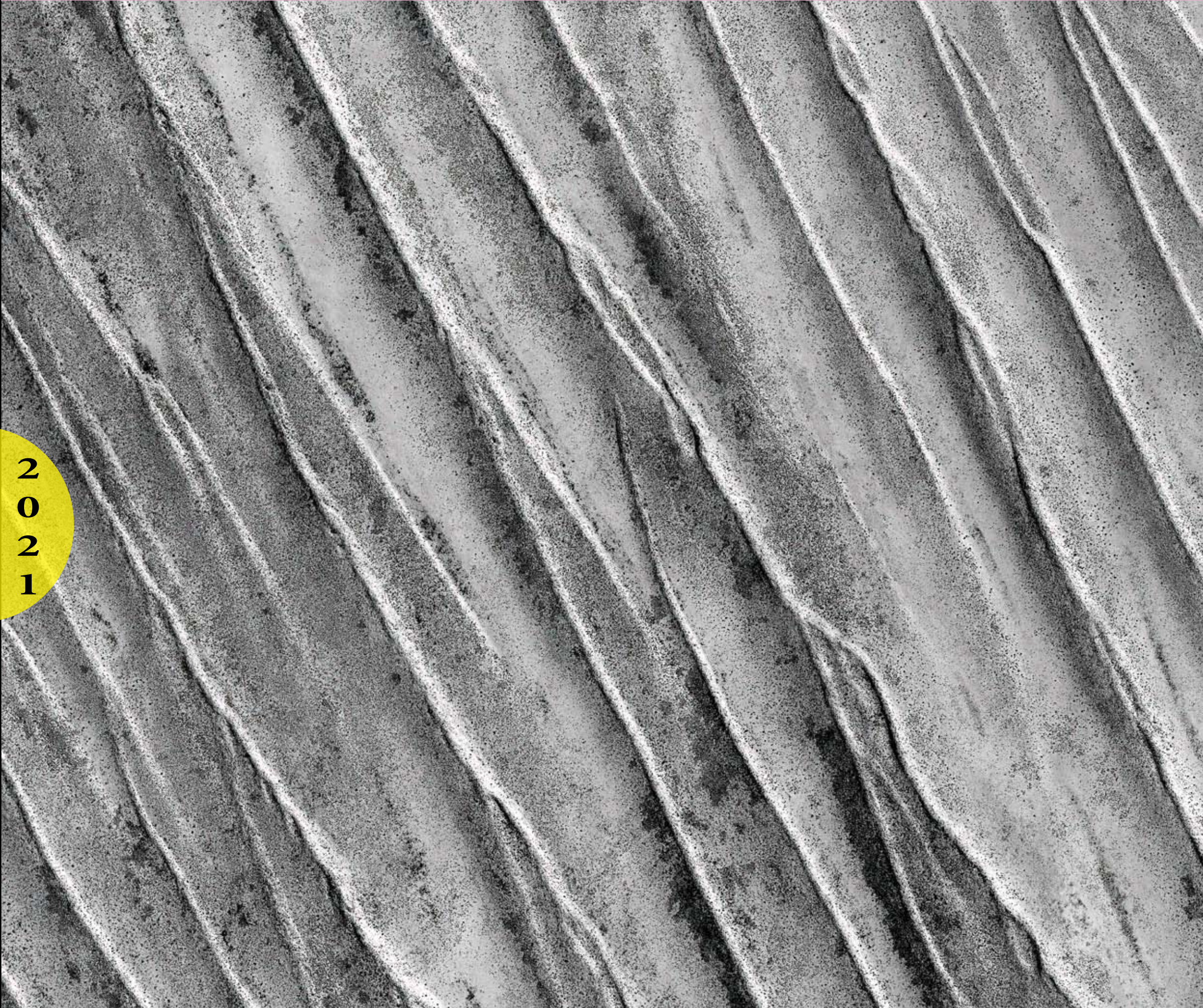
Spectacular longitudinal dunes in Simpson Desert, Australia. They have developed by helicoidal wind flow of the prevailing south-southeastern winds, acting upon ancient alluvial plains.
